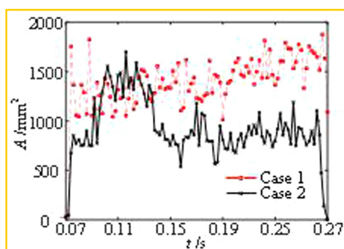
FIG. 11. Areas of the chemical reaction zones (OH) with varying jet locations and \phi = 0.3 .
