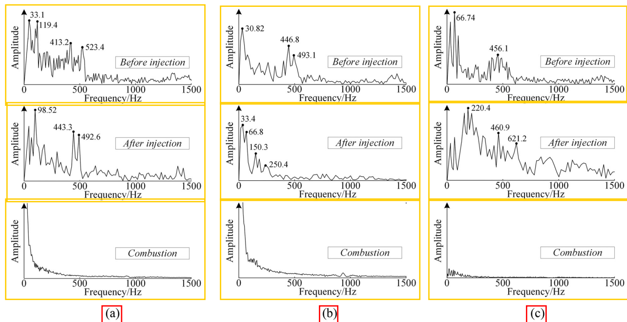
FIG. 20. FFT analysis of pressure–time history at x = 371 mm: (a) FFT analysis result of case 1; (b) FFT analysis result of case 2; and (c) FFT analysis result of case 6.
