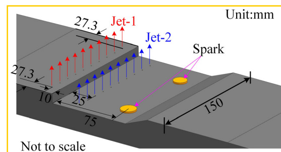
FIG. 3. Schematic of fuel injection and spark.
