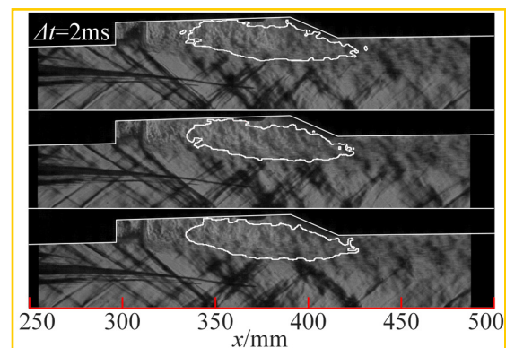
FIG. 18. Schlieren images and the CH region without H_2 pilot flame.
