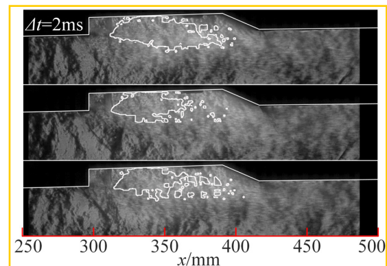
FIG. 17. Schlieren images and the CH region in the presence of the H_2 pilot flame.
